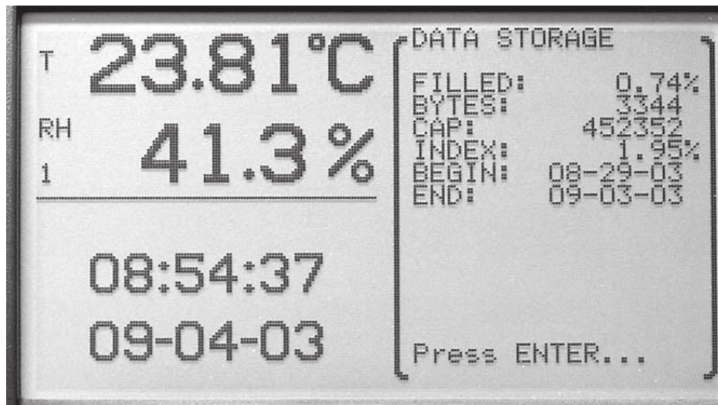
Figure 27 Data Storage
