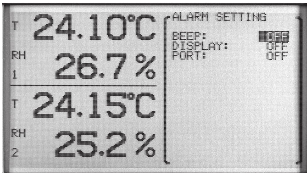
Figure 35 Alarm Setting
