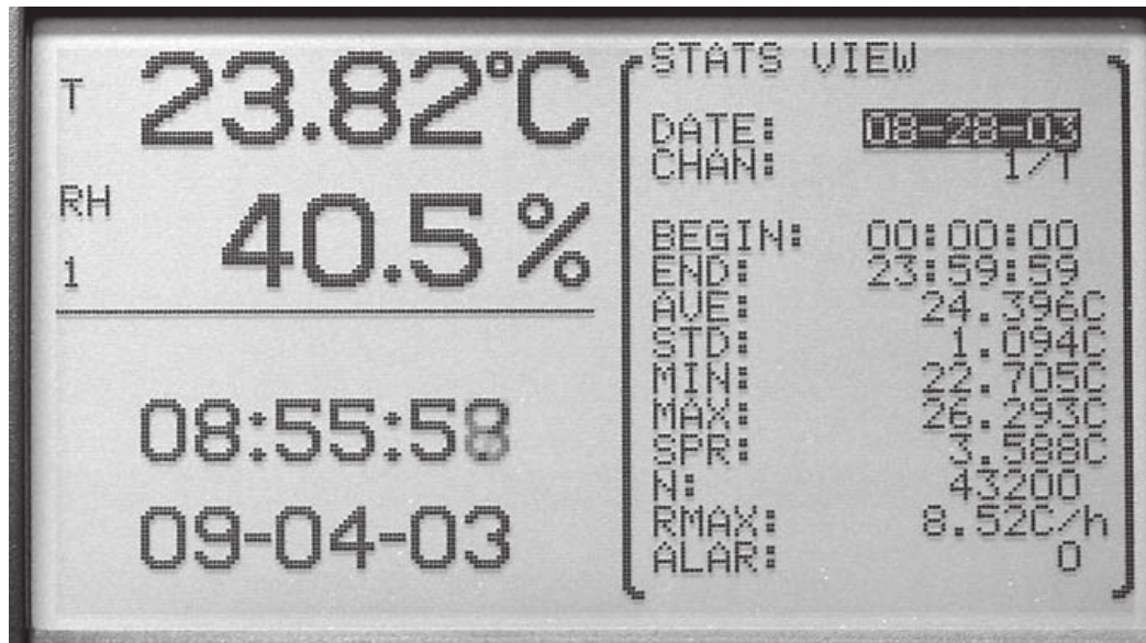
Figure 30 Stats View
