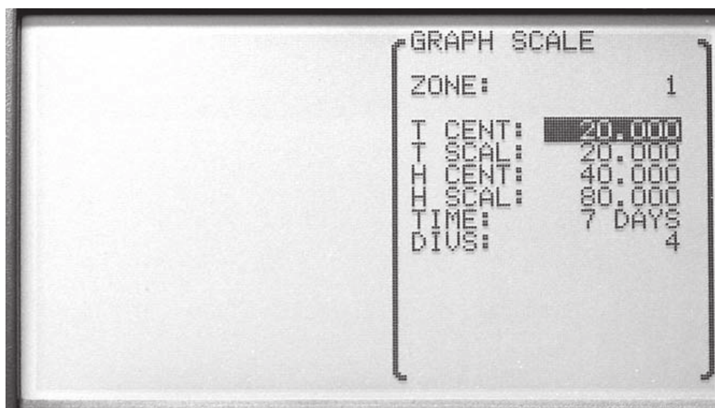
Figure 17 Graph Scale
