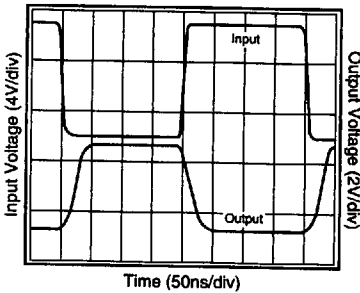
Figure 5: Overdrive Recovery
