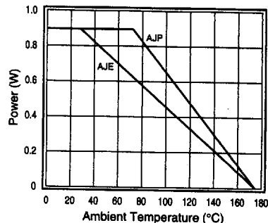
Figure 7: Power Derating Curves
