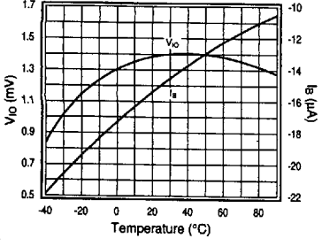
I_b , V_{io} , vs. Temperature
