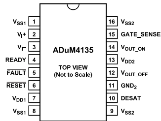
Figure 3. Pin Configuration
