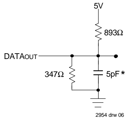
Figure 2. Output Test Load
