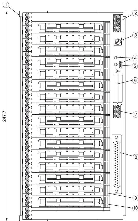
Figure 1 Structure
