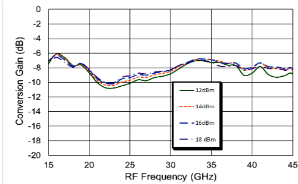
Down Conversion Gain over LO drive
