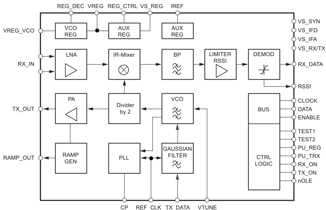
Figure 1-1. Block Diagram
