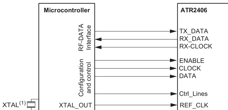
Figure 9-1. Microcontroller Interfacing with General Purpose MCU, Pin Connections between Microcontroller and ATR2406
