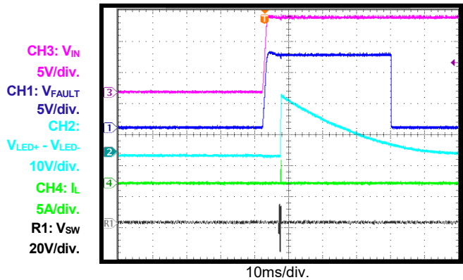
No Dimming LED open, start-up through VIN
