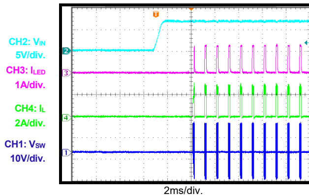
Two-Step Dimming Start-Up through V_{IN}
