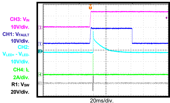
PWM Dimming LED open, start-up through VIN
