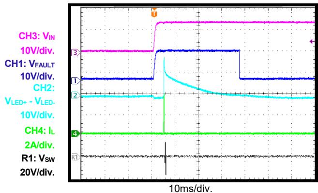
Two-Step Dimming LED open, start-up through VIN
