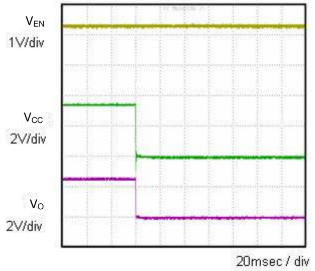
Fig.6 OFF sequence 1 C_o=1\mu\text{F}
