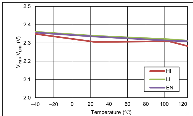
Figure 20. HI/LI/EN Pin High Threshold vs Temperature
