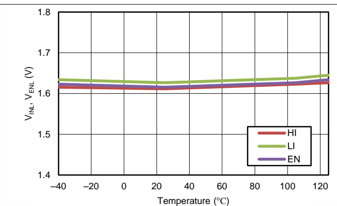
Figure 21. HI/LI/EN Pin Low Threshold vs Temperature
