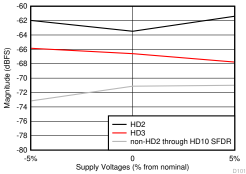
All supplies changed together, high power mode Figure 8-61. HD2, HD3 and Worst non-HD Spur vs Supply Voltage
