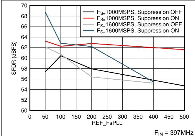
Figure 8-39. SFDR vs F_{REF} and Suppression
