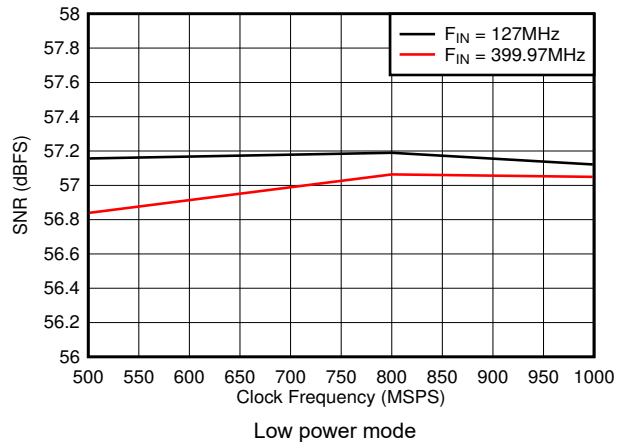
Figure 8-28. SNR vs Sample Rate
