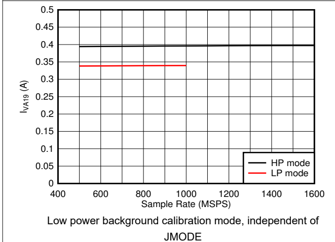
Figure 8-93. Dual Channel, I_{VA19} vs F_S
