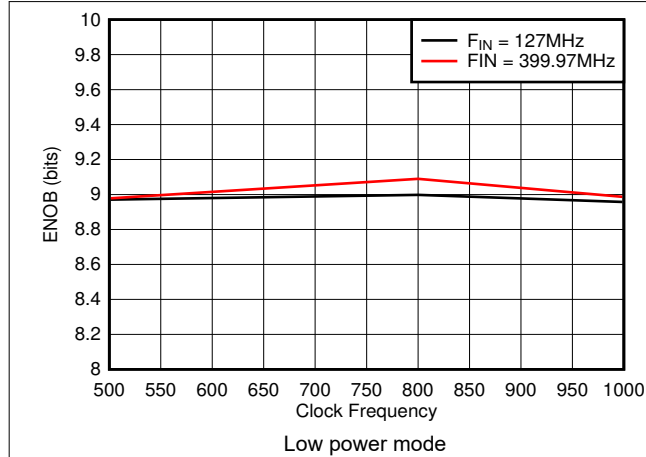
Figure 8-31. ENOB vs Sample Rate
