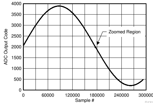
Figure 8-126. Background Calibration Core Transition (AC Signal)
