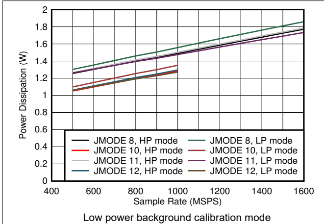
Figure 8-91. Dual Channel, Power Dissipation vs F_S and JMODE 8 - 12
