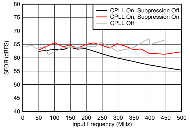
Figure 8-44. SFDR vs F_{IN} and C-PLL modes
