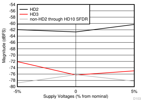
All supplies changed together, low power mode, F_S = 1000 MSPS Figure 8-63. HD2, HD3 and Worst non-HD Spur vs Supply Voltage
