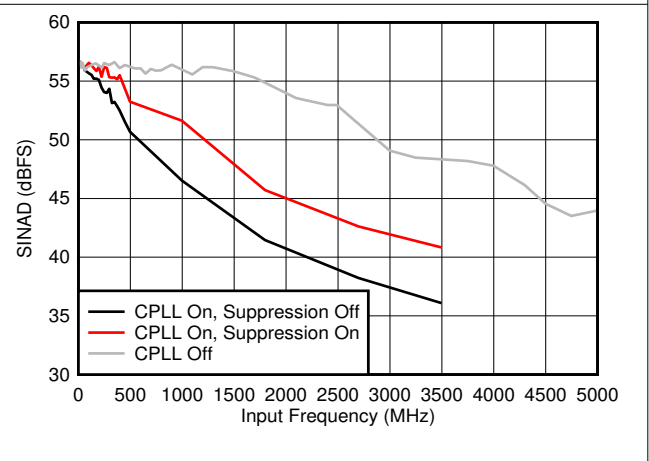
Figure 8-42. SINAD vs F_{IN} and C-PLL modes
