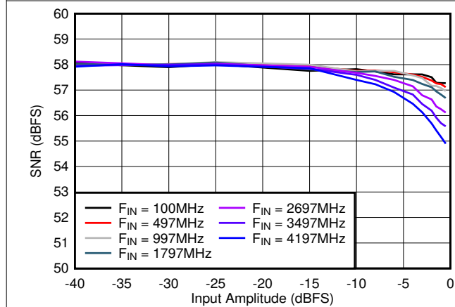
Figure 8-33. SNR vs A_{IN}
