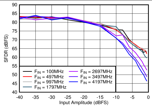
Figure 8-32. SFDR vs A_{IN}
