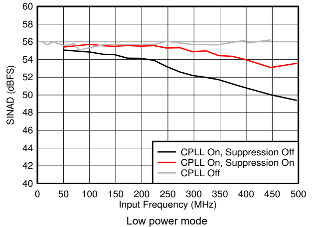
Figure 8-46. SINAD vs F_{IN} and C-PLL modes
