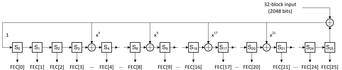
Figure 9-10. FEC Parity Bit Generator
