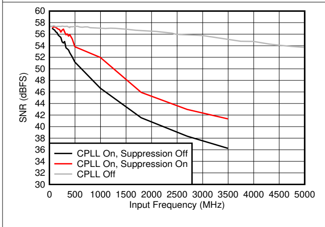
Figure 8-41. SNR vs F_{IN} and C-PLL modes
