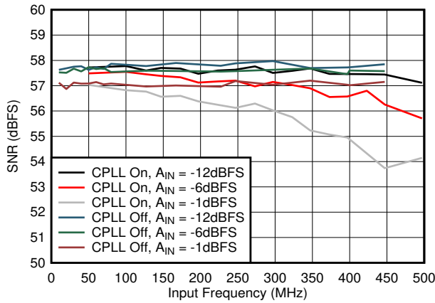
Figure 8-55. SNR vs A_{IN} and C-PLL
