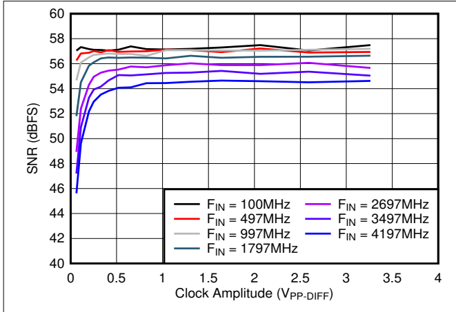
Figure 8-37. SNR vs A_{CLK}
