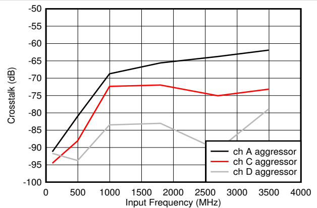
Figure 8-78. Crosstalk to Channel B vs F_{IN}
