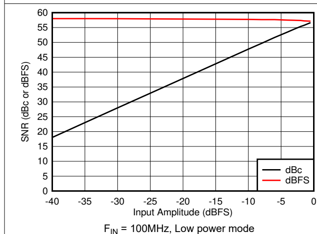
Figure 8-35. SNR vs A_{IN}
