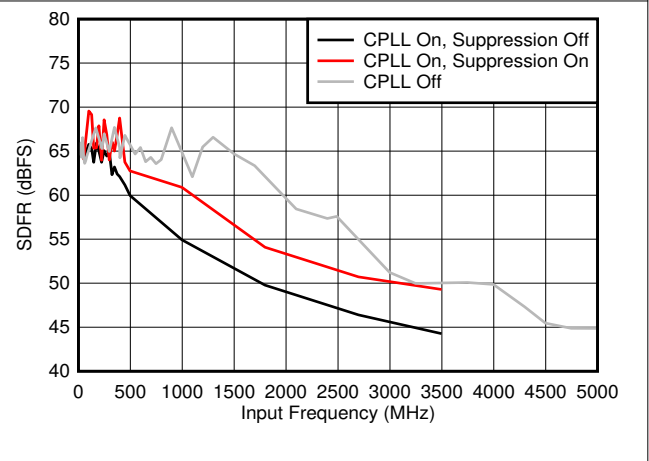
Figure 8-40. SFDR vs F_{IN} and C-PLL modes
