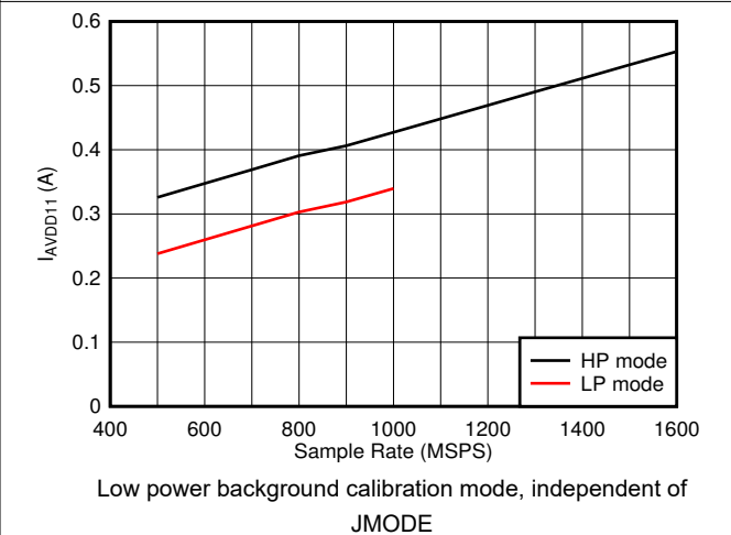
Figure 8-94. Dual Channel, I_{VA11} vs F_S
