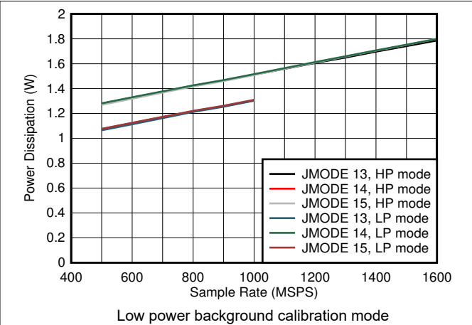
Figure 8-92. Dual Channel, Power Dissipation vs F_S and JMODE 13 - 15
