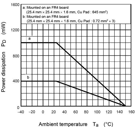
Fig. 8.14 P_D - T_a
