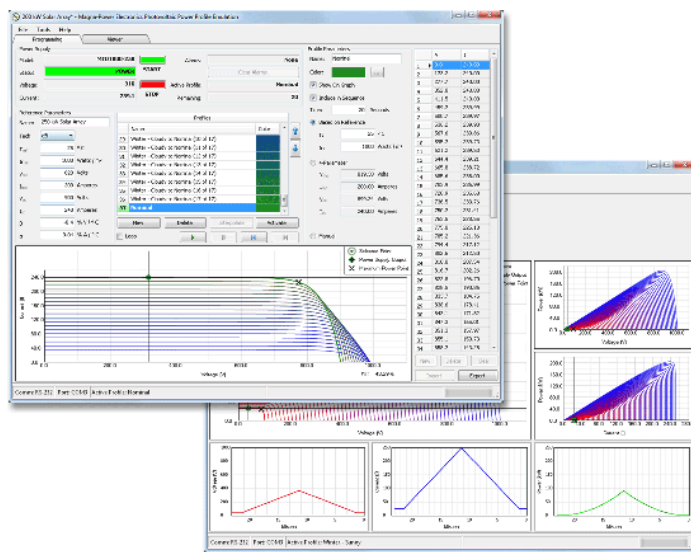
Magna-Power Electronics Photovoltaic Power Profile Emulation (PPPE) software: main programming window (foreground); Viewer window (background)
