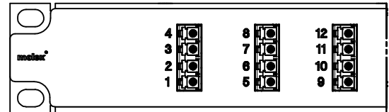
FRONT VIEW OF PANEL WHERE LC QUAD ADAPTERS ARE MOUNTED
