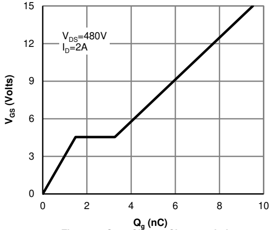
Figure 7: Gate-Charge Characteristics
