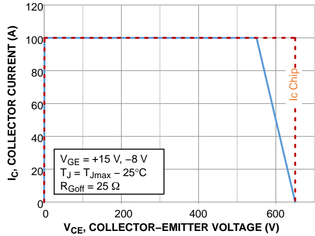
Figure 28. IGBT RBSOA
