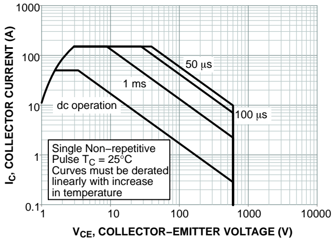
Figure 27. IGBT FBSOA
