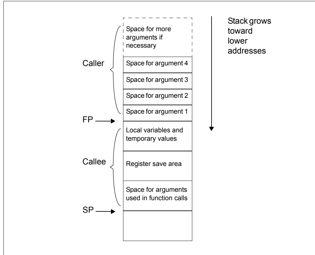
FIGURE 9-1: STACK FRAME
