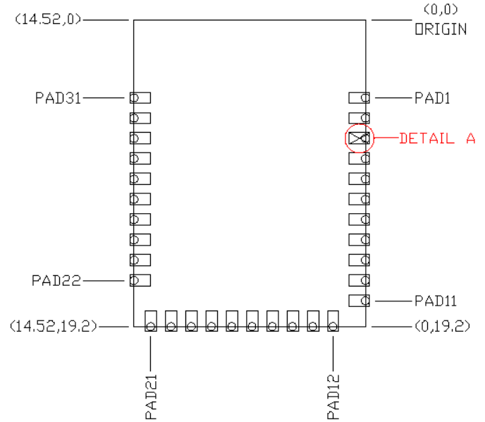
Top View (Seen on Host PCB)
