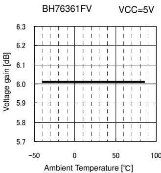
Fig.34 G v vs. Ambient Temperature
