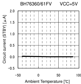
Fig.26 ICC2 vs. Ambient Temperature
