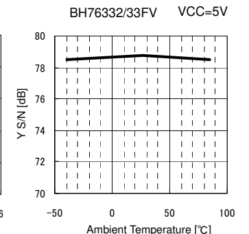
Fig.96 SN_V vs. Ambient Temperature
