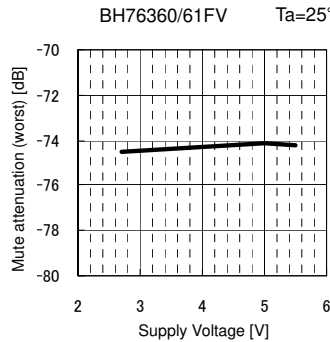
Fig.43 MT(worst) vs. Supply Voltage
