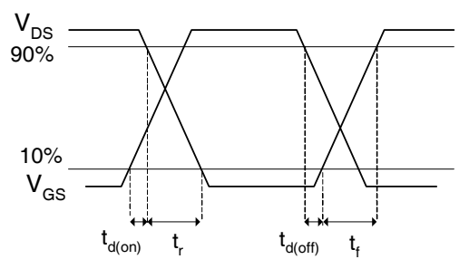
Fig 20b. Switching Time Waveforms
