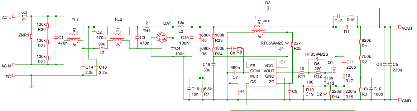
Figure 3. BD7693FJ-EVK-001 Schematics
