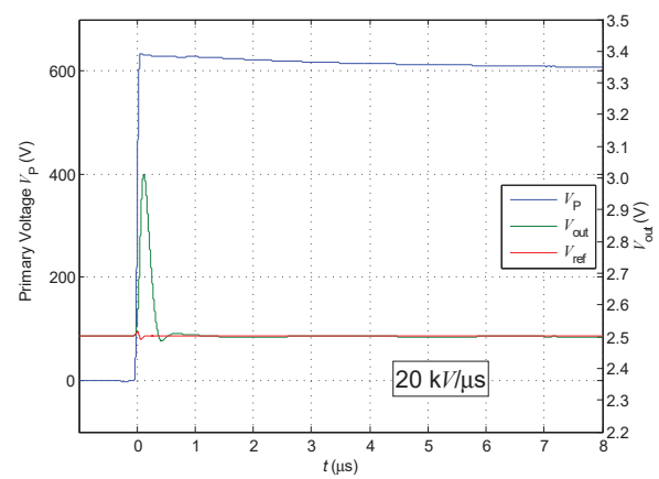
Figure 5: dv/dt
