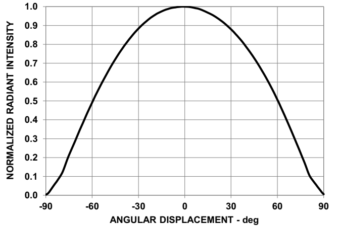
Figure 7: Radiation Pattern for AREQ-80C0-00000
