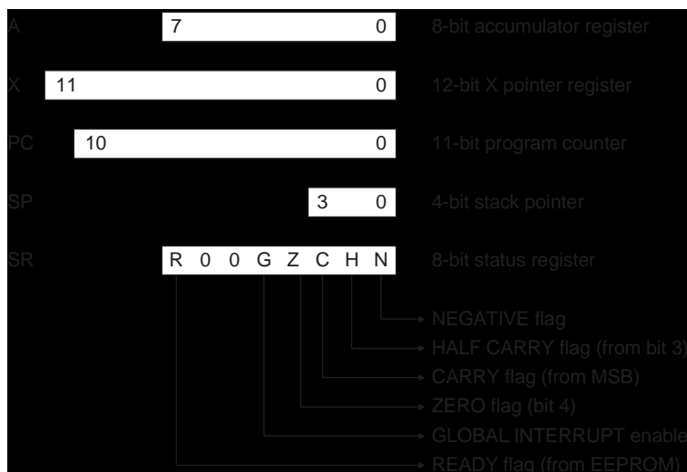
Figure 12. Programming Model
