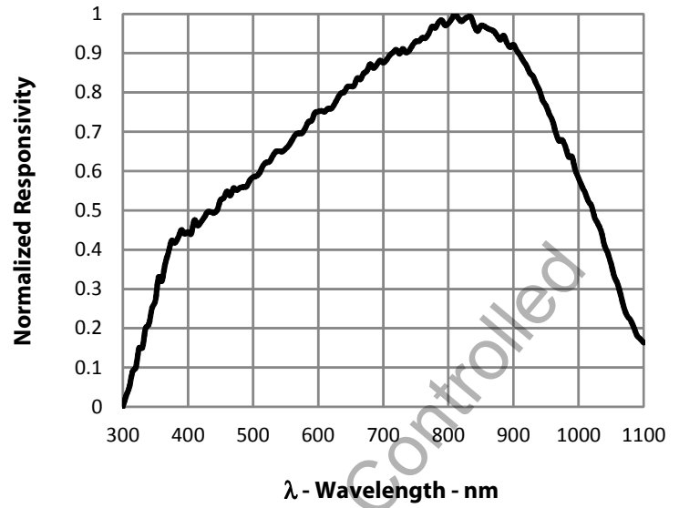
Figure 10: Spectral Responsivity
