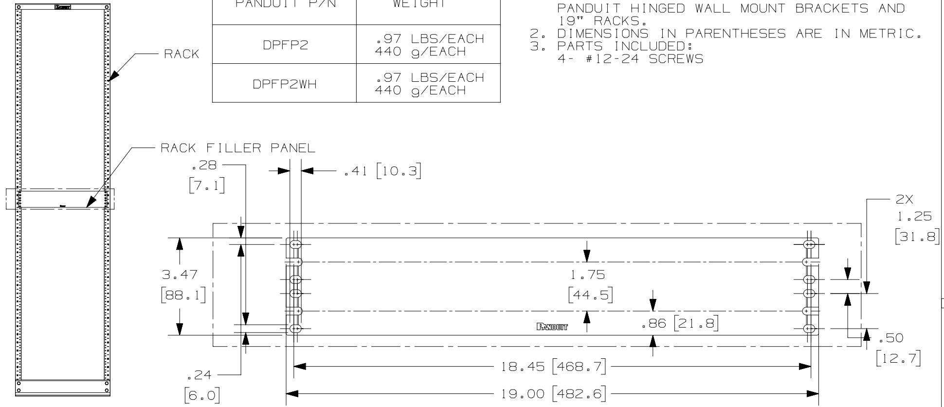
DETAIL VIEW
