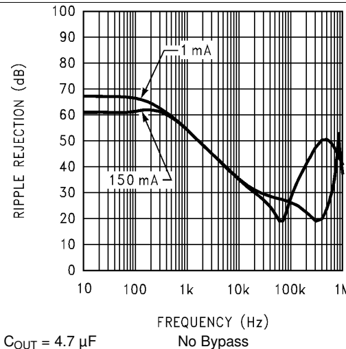
Figure 6. Ripple Rejection
