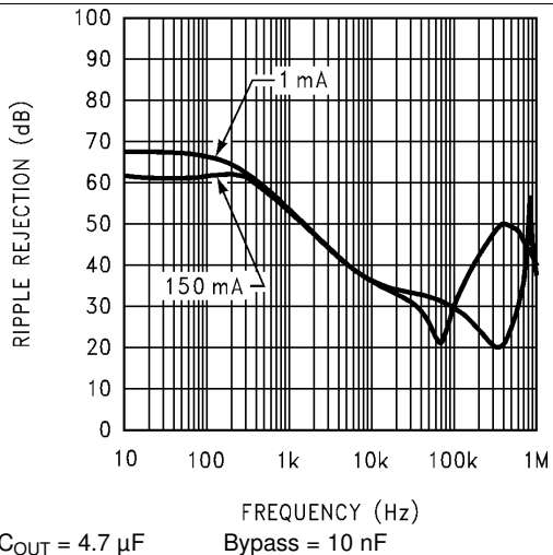
Figure 5. Ripple Rejection
