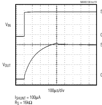
MAX6138_50 STARTUP CHARACTERISTICS
