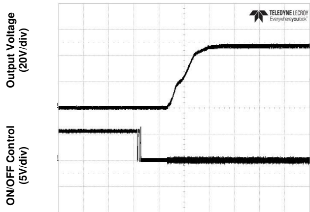
Figure 4. Start-Up from Enable Control (typical Vin, full load, 1,000µF external output capacitance)
