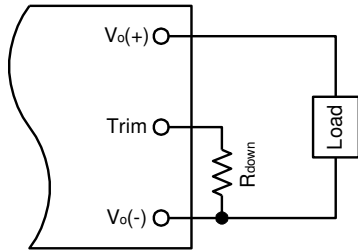
Figure 13. Circuit to Decrease Output Voltage
