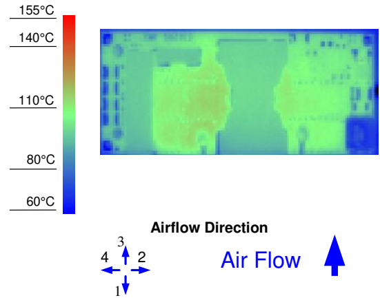
Figure 8. Thermal Image for Airflow Direction 3 (17A output, 55°C ambient, 200 LFM, typical Vin, open frame unit)
