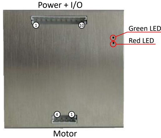
Figure 8: TMCM-1276 connectors
