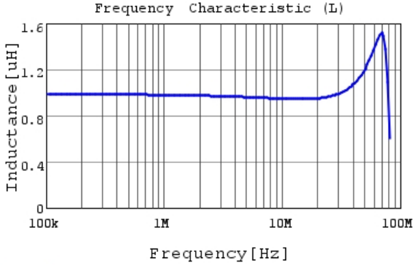
DFE2MCAH1R0MJ0 L
