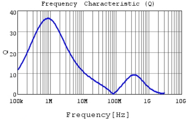
DFE2MCAH1R0MJ0 Q
