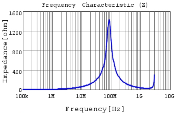
DFE2MCAH1R0MJ0 |Z|
