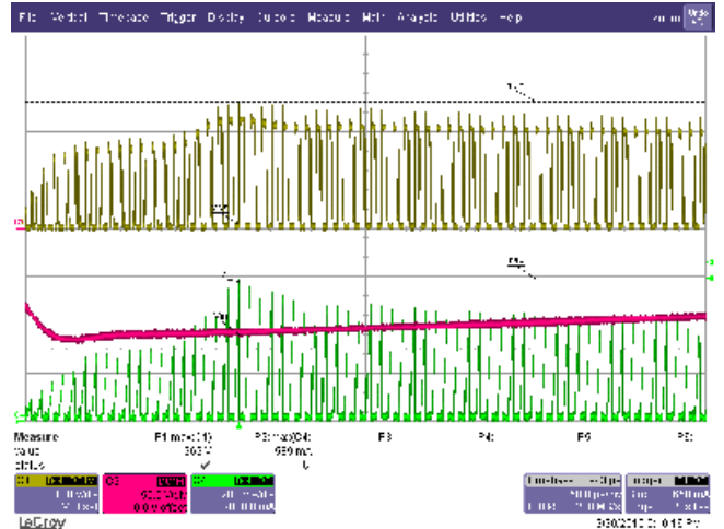
Figure 40 – 115 VAC / 60 Hz, 135° Dimming Phase Angle. 6 LED in Series (18.2 V / 350 mA) Ch1(Yellow): V_{DS} , 100 V / div. Ch2(Red): V_{IN} , 50 V / div. Ch4(Green): I_{DS} , 200 mA / div., 50 \mu s / div.
