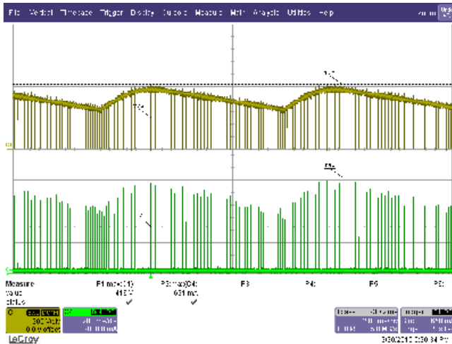
Figure 47 – 265 VAC. Load Shorted. Upper: V_{DRAIN} , 200 V / div. Lower: I_{DRAIN} , 0.2 A / div., 2 ms / div.
