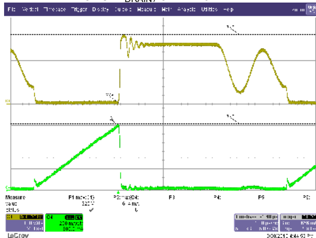
Figure 28 – 115 VAC / 60 Hz, 6 LED in Series (18.2 V / 350 mA). Upper: V_{DRAIN} , 100 V / div., 1 µs / div. Lower: I_{DRAIN} , 0.2 A / div.
