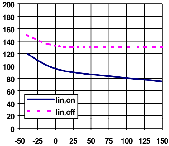
Figure 17 - Inputcurrent (mA) Vs Junction (°C)
