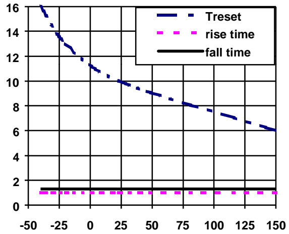
Figure 18 - Turn-on, Turn-off and Treset (ns) Vs Tj (°C)
