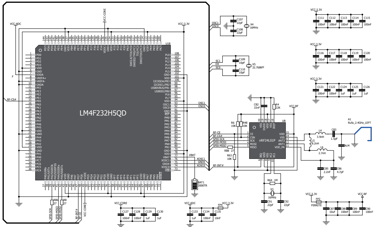
Figure 13-3: RF transceiver module schematic
