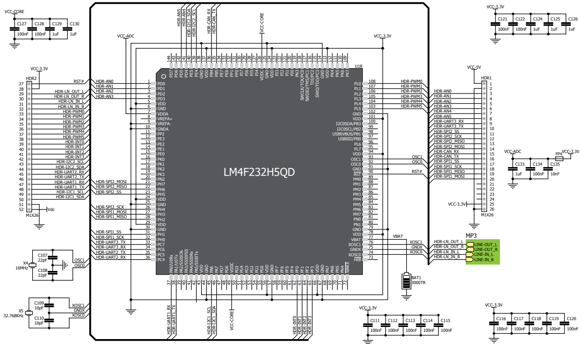
Figure 16-1: Connecting pads schematic
