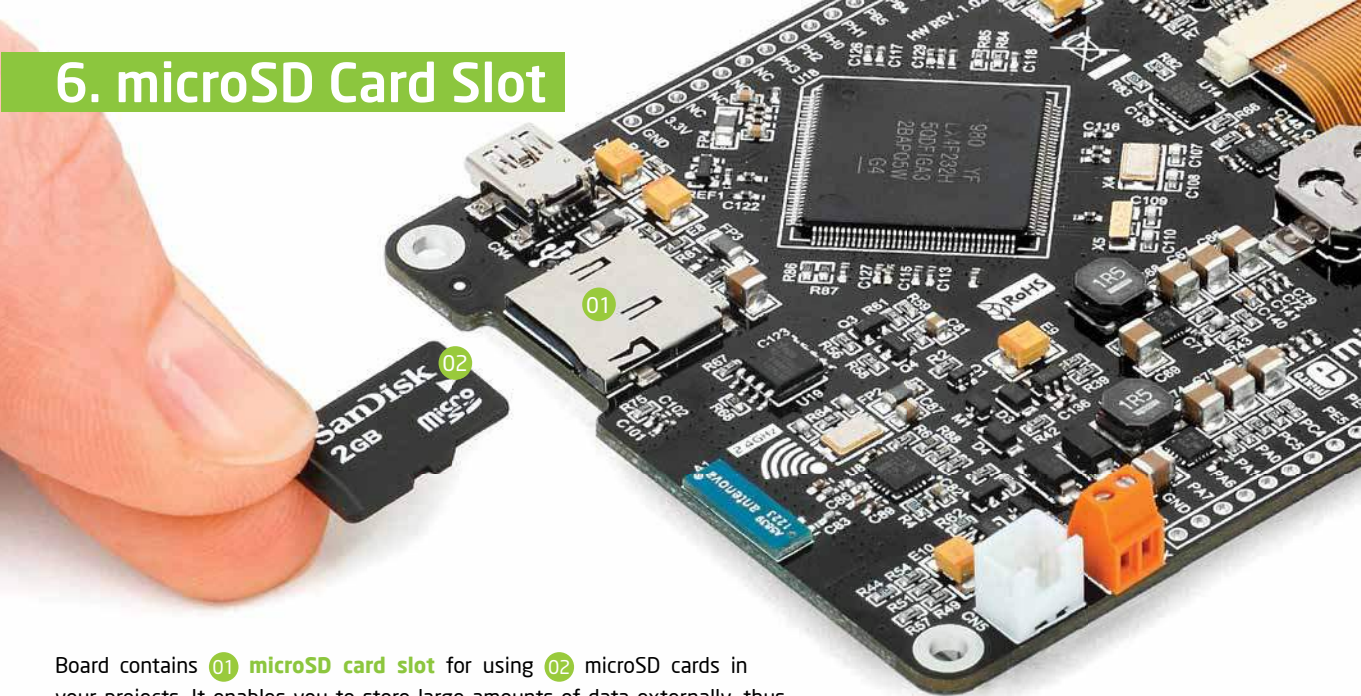
Figure 6-1: microSD card slot
