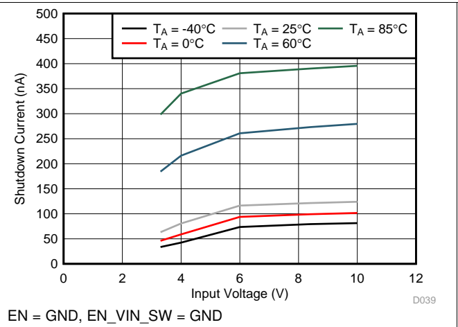
Figure 2. Shutdown Current
