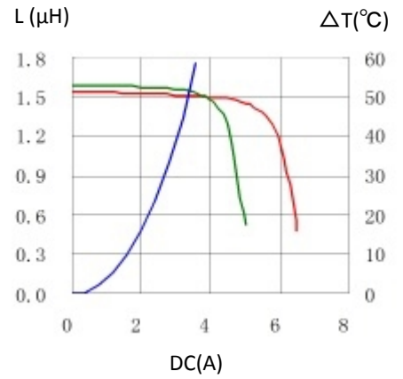
3. CD43T125NP-1R8MC
