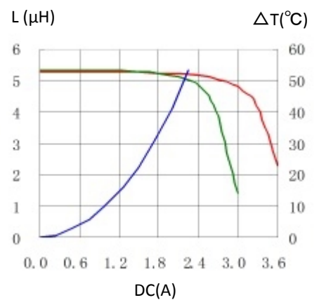
9. CD43T125NP-5R6MC
