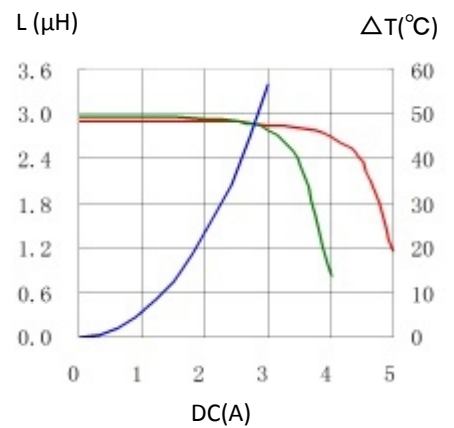
6. CD43T125NP-3R3MC
