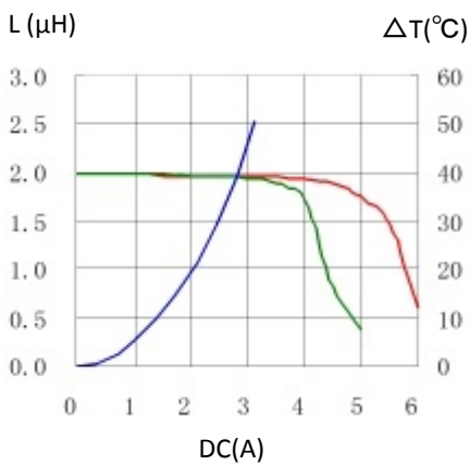
4. CD43T125NP-2R2MC
