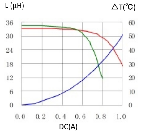
18. CD43T125NP-330KC
