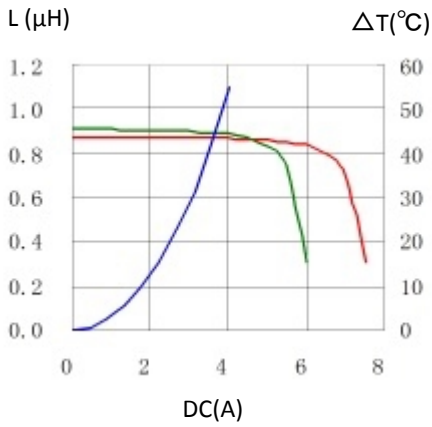
1. CD43T125NP-1R0MC
