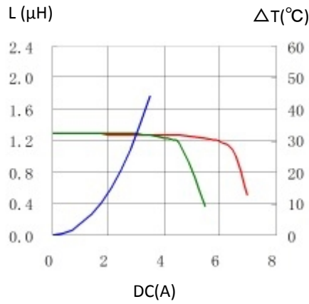
2. CD43T125NP-1R4MC
