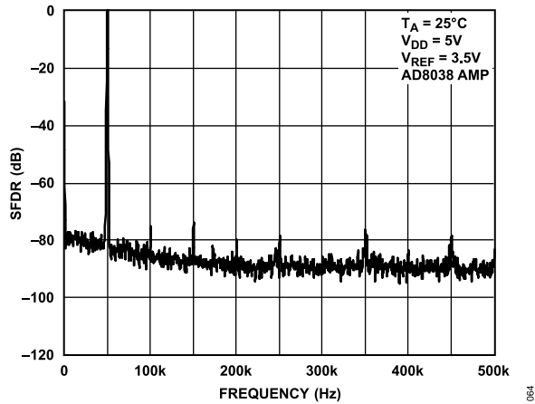
Figure 31. Wideband SFDR, f_{OUT} = 50 kHz, Clock = 1 MHz
