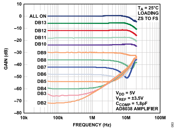
Figure 22. Reference Multiplying Bandwidth vs. Frequency and Code
