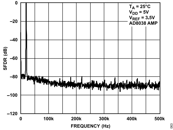
Figure 30. Wideband SFDR, f_{OUT} = 20 kHz, Clock = 1 MHz
