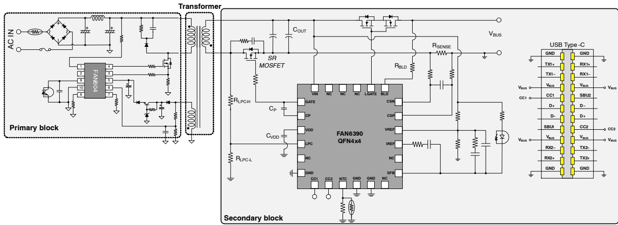
Figure 1. Application Schematic
