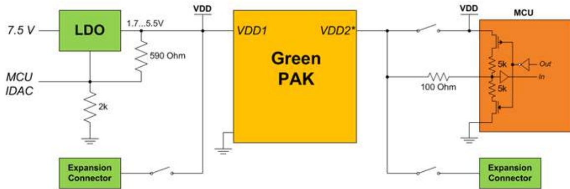
Figure 6: Schematic Connection of the V DD Pin
