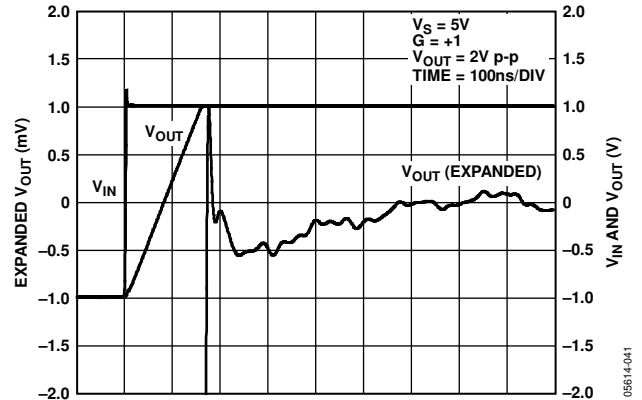
Figure 28. Settling Time
