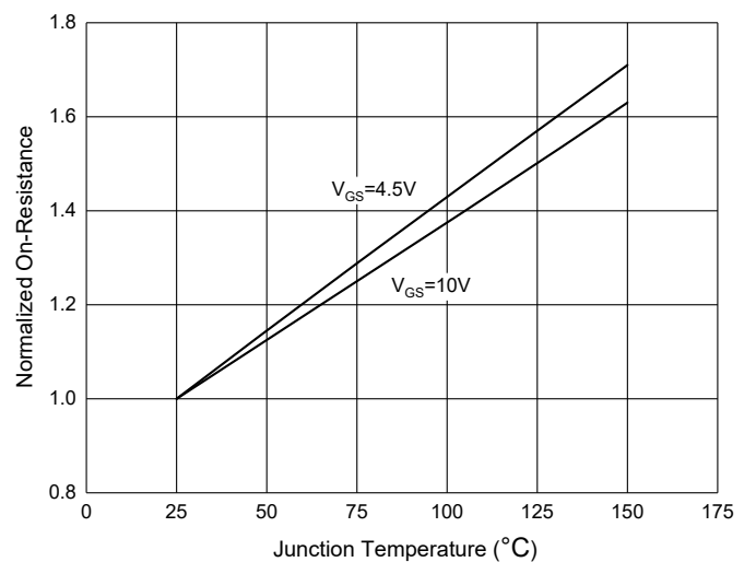
Fig. 6 - R_{DS(ON)} - \text{Temperature}
