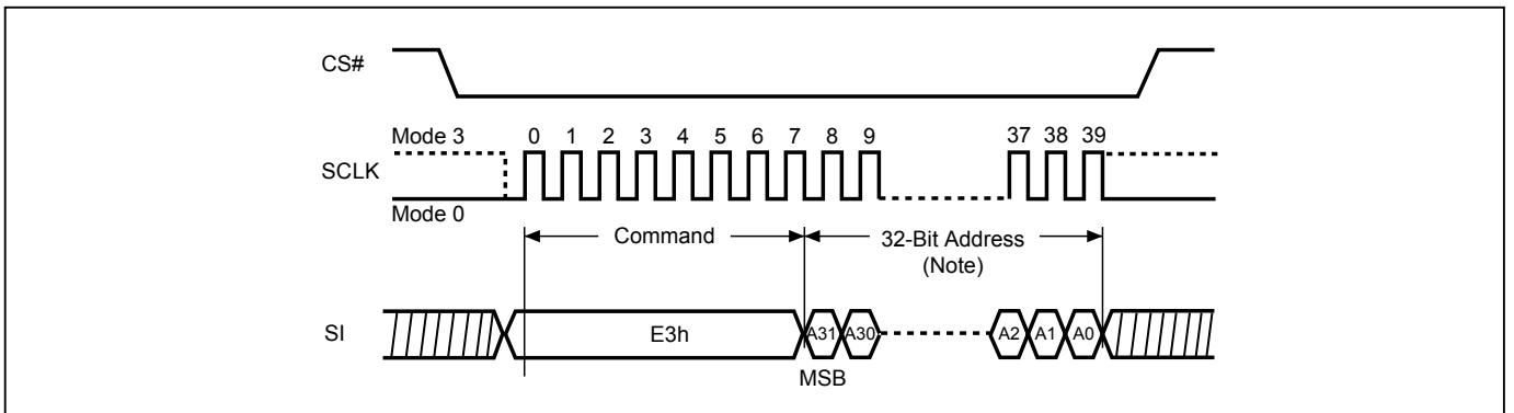
Figure 66. SPB Program (WRSPB) Sequence
