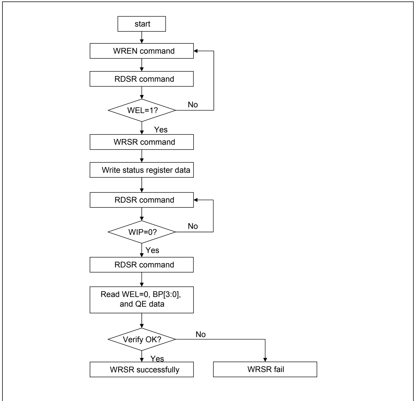
Figure 25. WRSR flow
