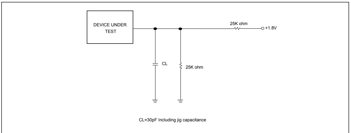
Figure 80. OUTPUT LOADING
