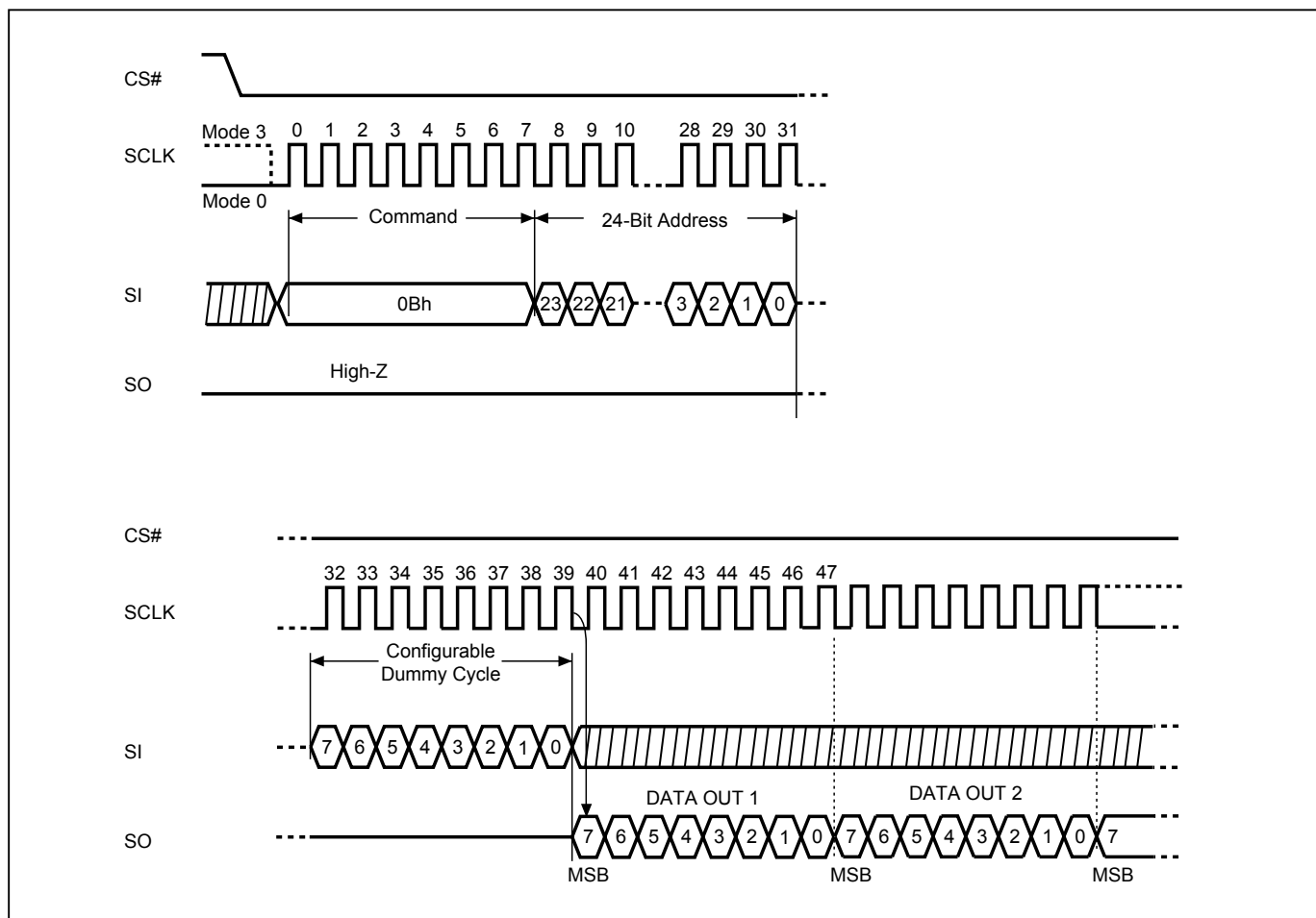
Figure 27. Read at Higher Speed (FAST_READ) Sequence (SPI Mode only)
