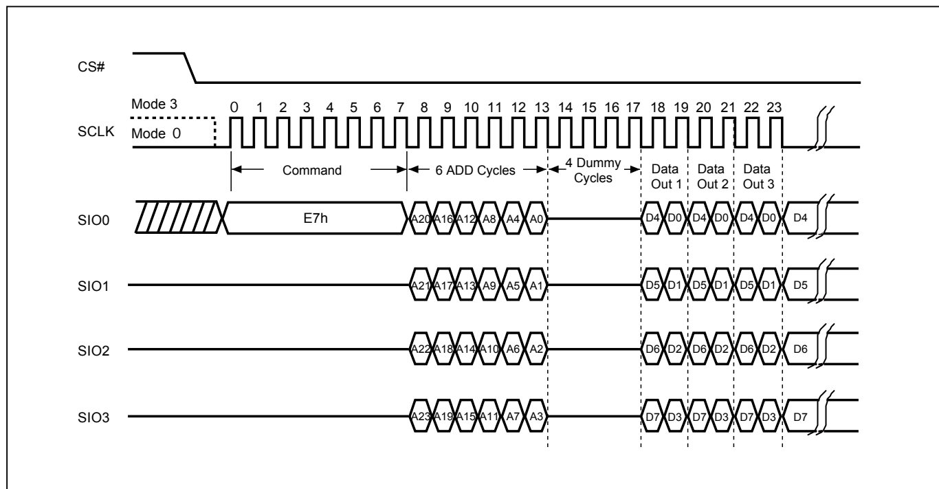
Figure 31. W4READ (Quad Read with 4 dummy cycles) Sequence (SPI Mode only)
