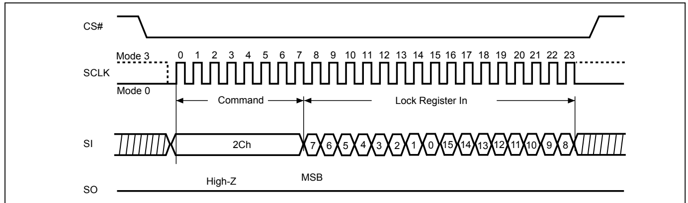
Figure 63. Write Lock Register (WRLR) Sequence
