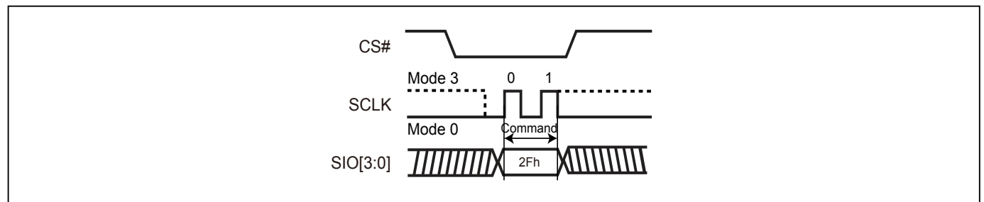
Figure 58. Write Security Register (WRSCUR) Sequence (QPI Mode)
