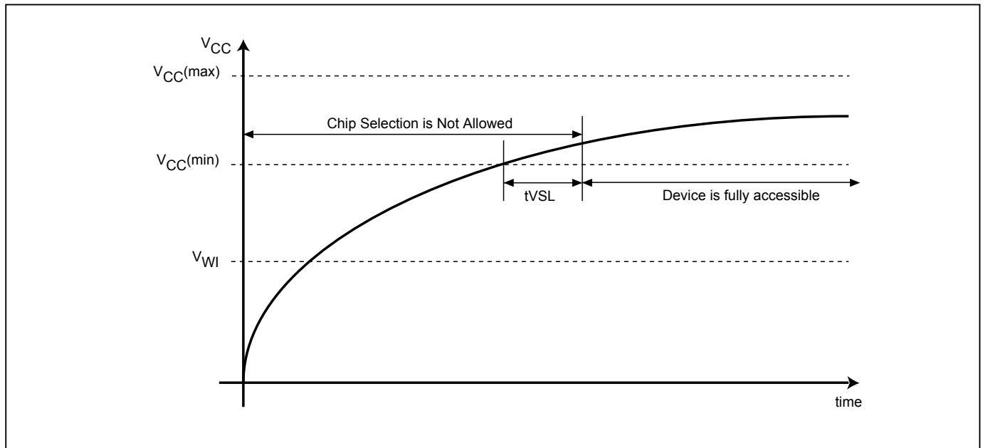
Figure 84. Power-up Timing
