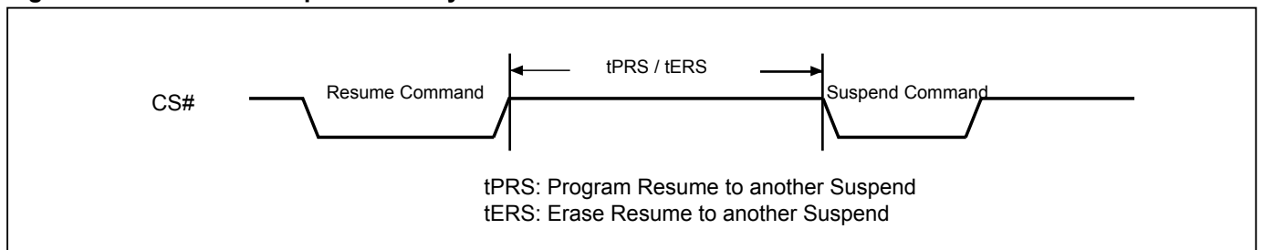
Figure 72. Resume to Suspend Latency
