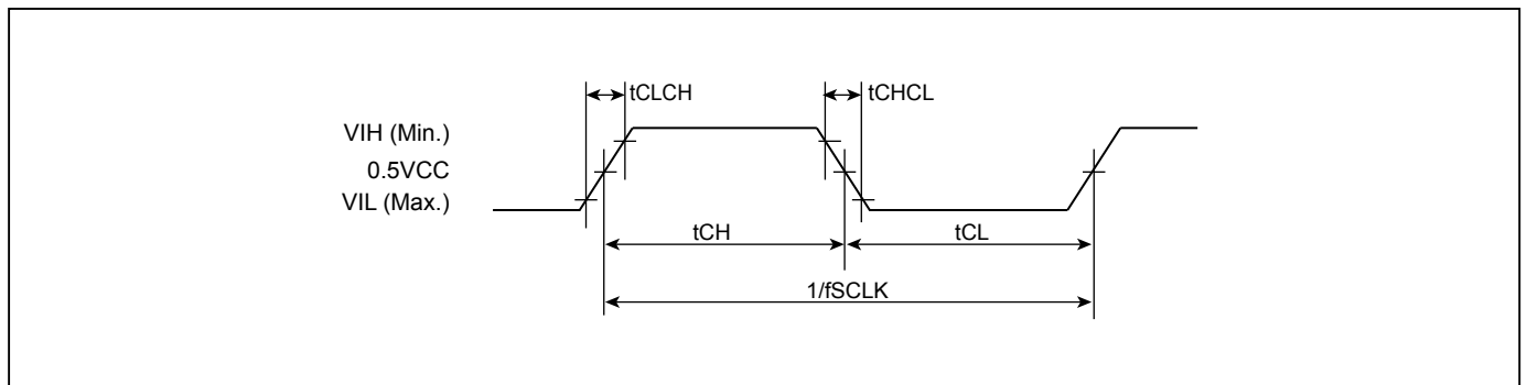
Figure 81. SCLK TIMING DEFINITION
