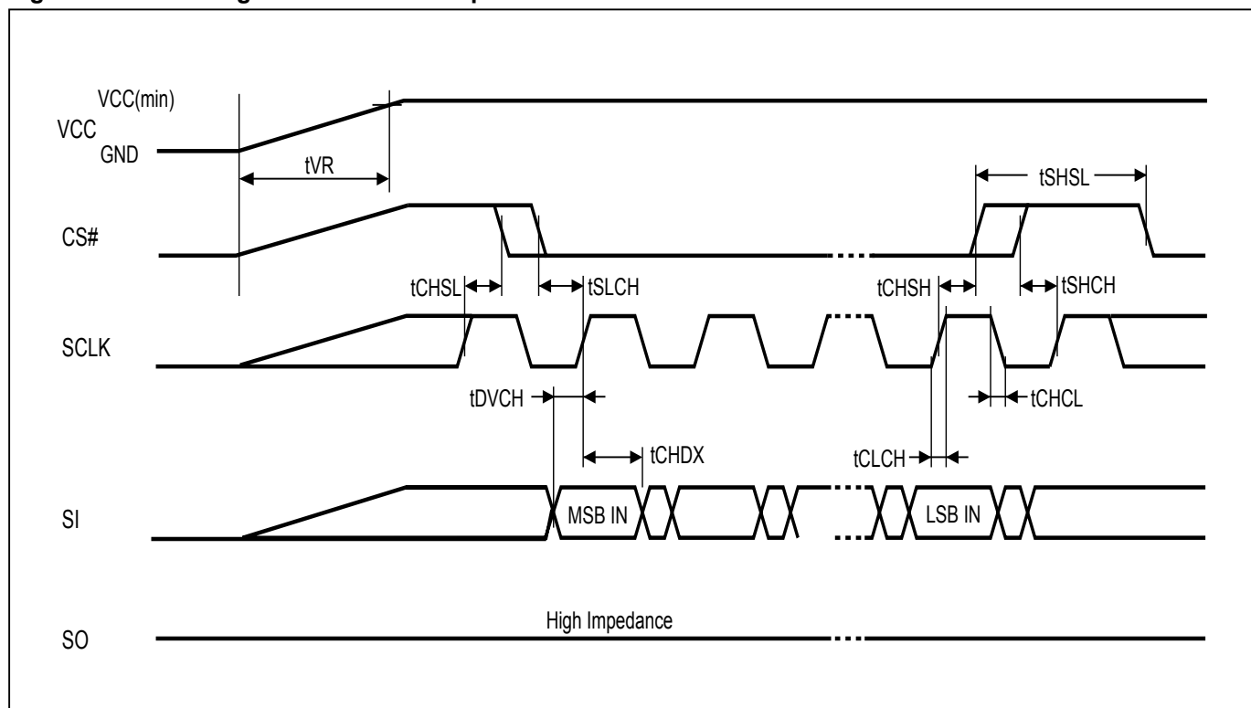
Figure 82. AC Timing at Device Power-Up
