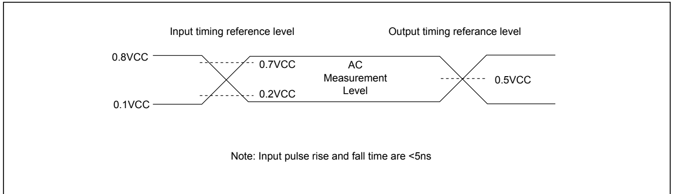
Figure 79. DATA INPUT TEST WAVEFORMS AND MEASUREMENT LEVEL
