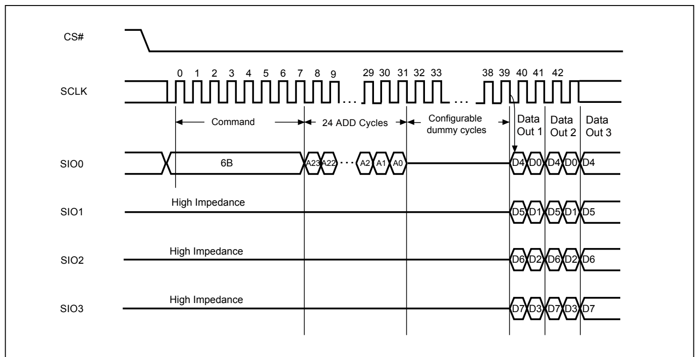
Figure 30. Quad Read Mode Sequence (SPI Mode only)
