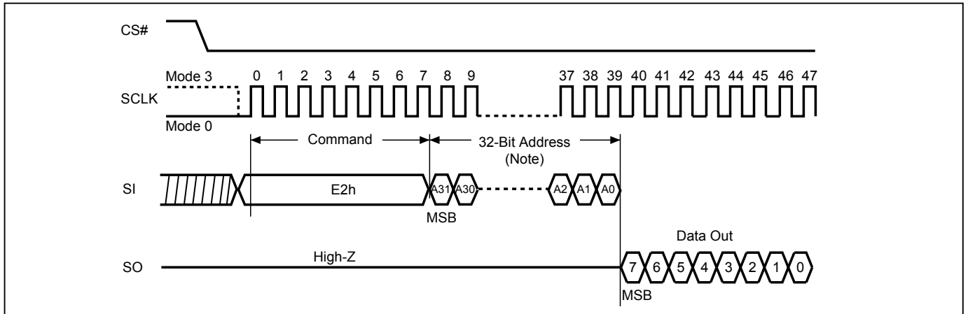
Figure 64. Read SPB Status (RDSPB) Sequence
