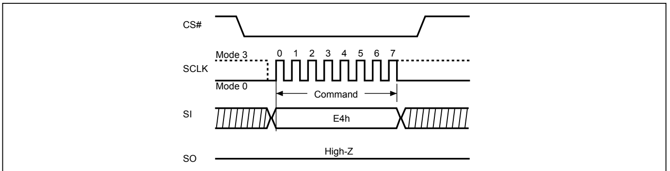
Figure 65. SPB Erase (ESSPB) Sequence
