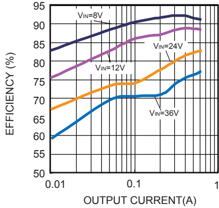
Efficiency V_{OUT}=5V
