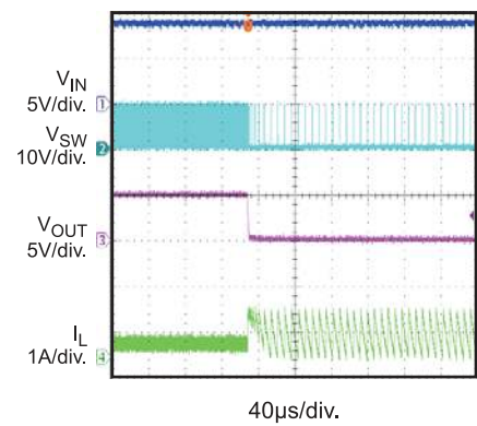
Short Output
