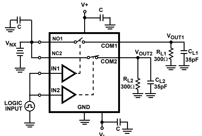
FIGURE 2. CHARGE INJECTION
