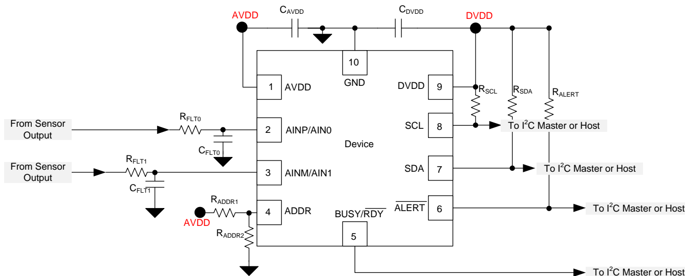
Figure 123. Example Circuit
