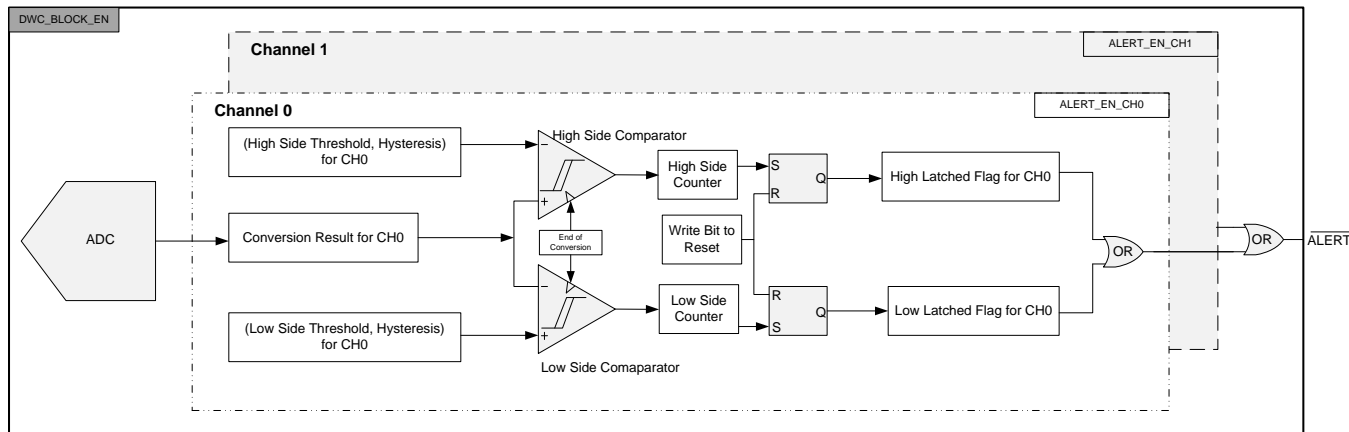
Figure 47. Digital Comparator Block Diagram
