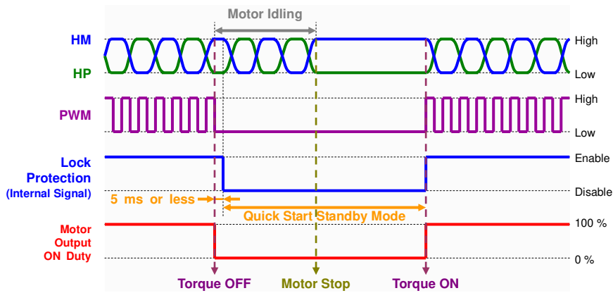
Figure 22. Quick Start Timing Chart
