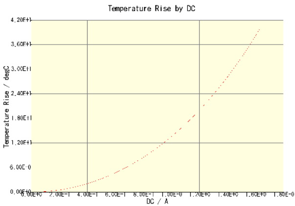
CLF7045T-470M-CA(Amb. Temp. = 20degc)
