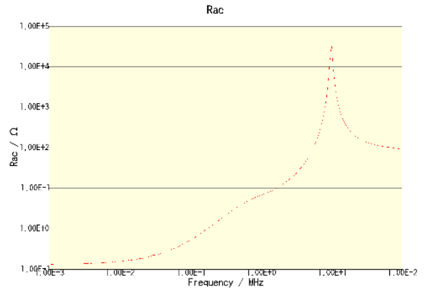
CLF7045T-470M-CA
