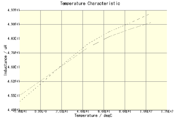
CLF7045T-470M-CA(DC = 0A)
