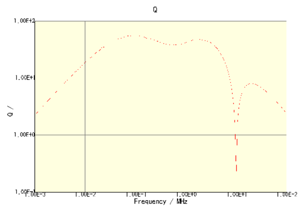
CLF7045T-470M-CA
