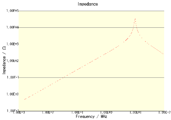
CLF7045T-470M-CA
