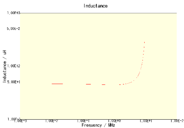
CLF7045T-470M-CA
