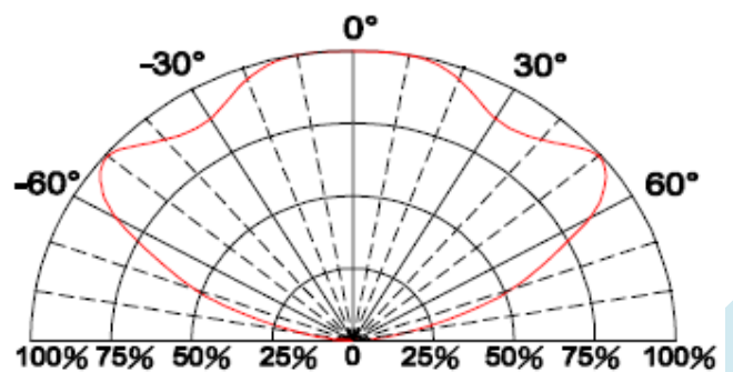
Fig.6 Directive Radiation
