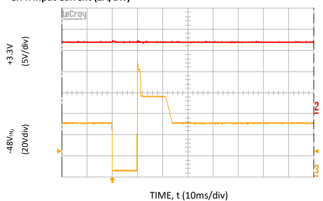
Fig 7b: Line Transient performance per ANSI T1.315-2001 standard vs 3.3V output
