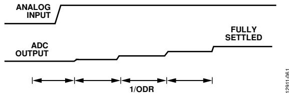
Figure 57. Step Input Without Single Cycle Settling
